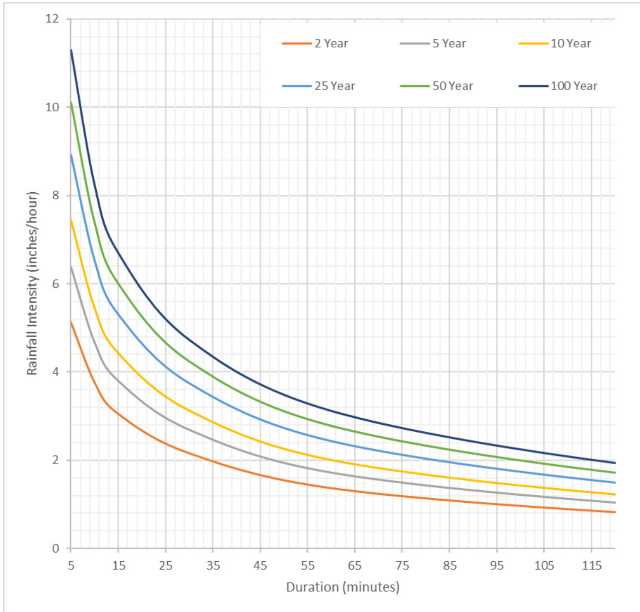
Figure 2-1. Intensity-Duration-Frequency Curves
