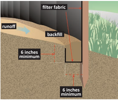
Fig. 3-4. Silt fence installation detail. Source: Utah DOT
