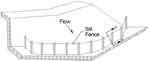
Fig. 3-2. Isometric view of a silt fence installation. Source: Colorado DOT
